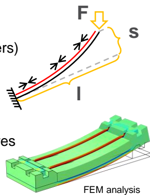
FEM analysis
